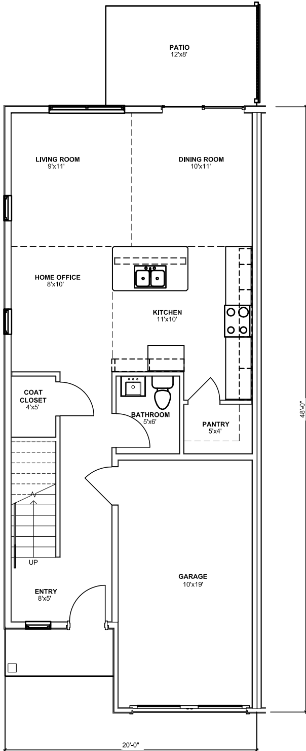
1 PLAN TYPE C END - FIRST FLOOR 1/4" = 1'-0"
