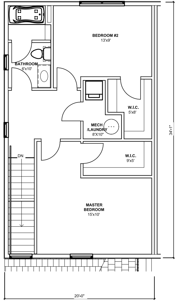
2 PLAN TYPE C END - SECOND FLOOR 1/4" = 1'-0"
