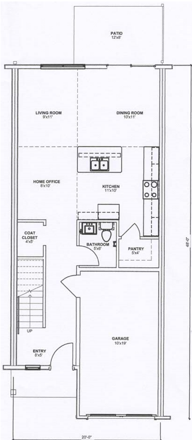
1 PLAN TYPE C MID - FIRST FLOOR 1/4" = 1'-0"
