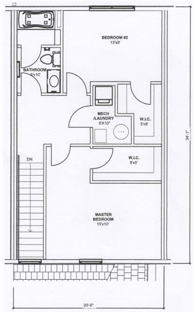
2 PLAN TYPE C MID - SECOND FLOOR 1/4" = 1'-0"
